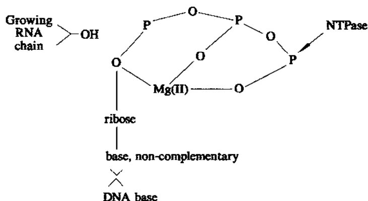
Fig. 1. Scheme for proposed mechanism of fidelity in RNA synthesis, showing a Mg(II) switch between conformers of RNA polymerase enzyme and substrate (see text).
